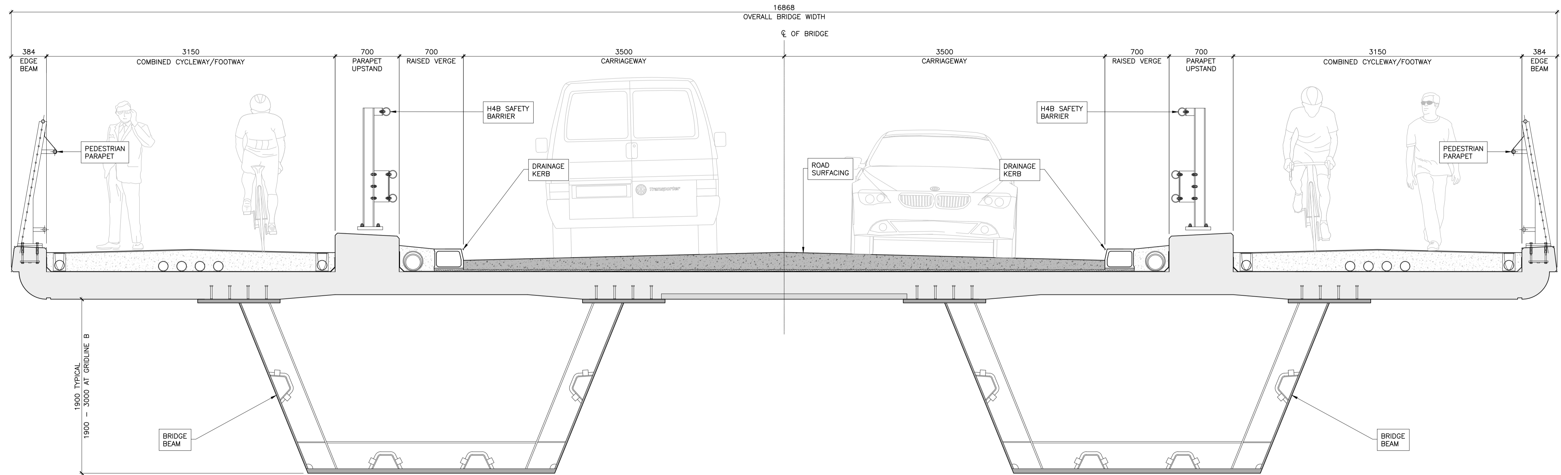
RIVER SLANEY BRIDGE TYPICAL DECK SECTION
