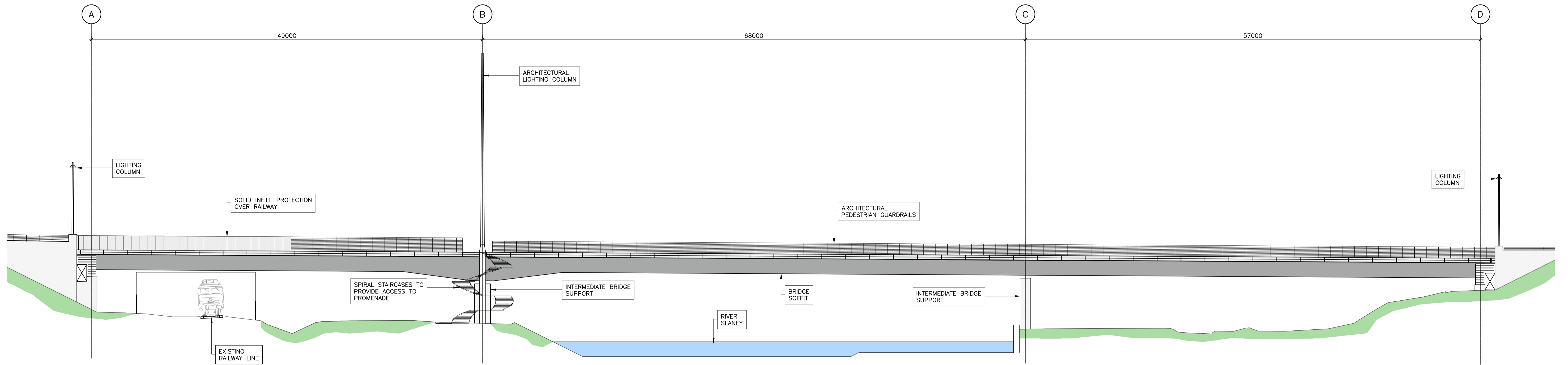
RIVER SLANEY BRIDGE ELEVATION FROM THE SOUTH
